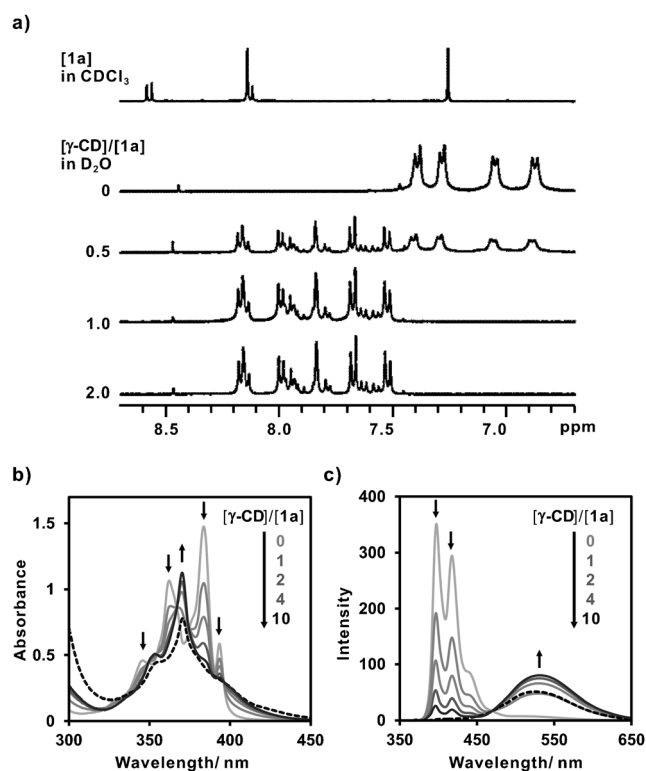
Figure 3. a) 1 H NMR spectra of 1a ( 3.0 \times 10^{-3} M) upon addition of increasing amounts of \gamma -CD at 25 °C in D 2 O. b) Absorption and c) fluorescence spectra of 1a ( 3.0 \times 10^{-5} M) upon addition of increasing amounts of \gamma -CD in H 2 O (gray and black line, respectively) and of [4]rotaxane 3 ( 1.5 \times 10^{-5} M, black dashed line) in a small amount of ammonia-containing H 2 O at ca. pH 9.5 at 25 °C. For (c), \lambda_{\text{ex}} = 370 nm.
